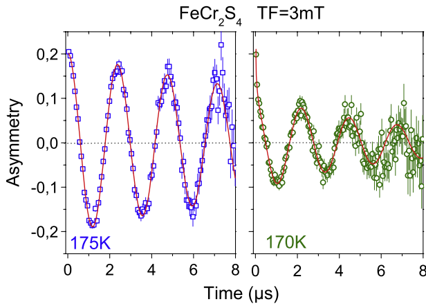
Figure 1. TF = 3 mT spectra of FeCr 2 S 4 above and near the magnetic ordering temperature. The solid lines are least squares fits to a single oscillatory signal (equation (2)) at 175 K with \chi^2 = 1.12 and to two signals (one oscillatory, the other a rapid exponential relaxation relevant at early times) at 170 K with \chi^2 = 1.06 . The origin of these different spectral functions is discussed in the text.
