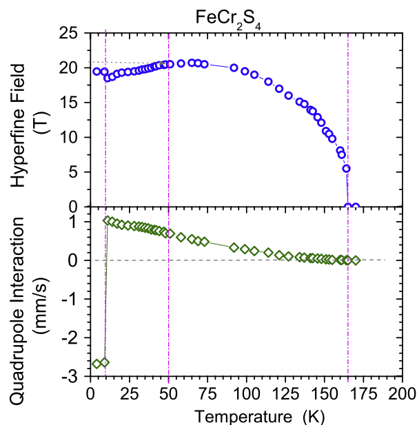
Figure 6. ^{57}\text{Fe} Mössbauer data of \text{FeCr}_2\text{S}_4 : Temperature dependences of the hyperfine field B_{\text{hf}} (top) and the quadrupole interaction (bottom). The solid lines are guides to the eye. The dash-dotted lines mark the temperature at which irregularities occur. The dotted line is the extrapolation of B_{\text{hf}} if no change at 50 K occurred.
