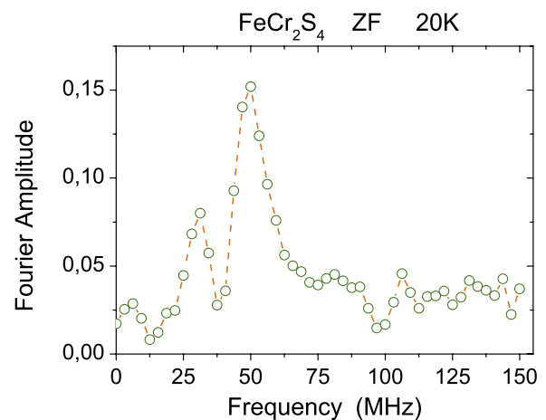
Figure 3. Fast Fourier transform of the ZF spectrum of FeCr 2 S 4 at 20 K. The line is a guide to the eye only.
